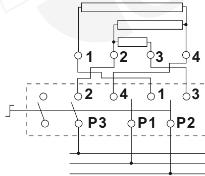
hot plate 2x3 connections 1x3-pole 4-position switch
