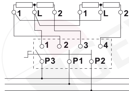
hot plate 2x3 connections 1x3-pole 4-position switch
