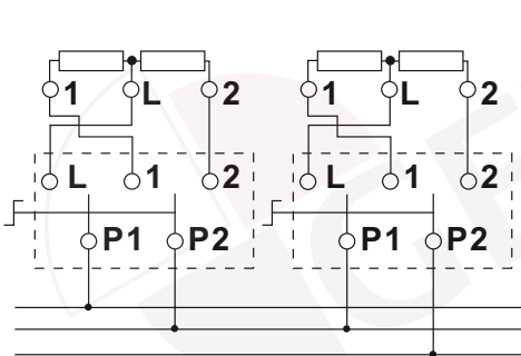
hot plate 2x3 connections 2x2-pole 4-position switch
