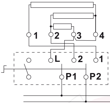
hot plate 4 connections 2-pole 5-position switch
