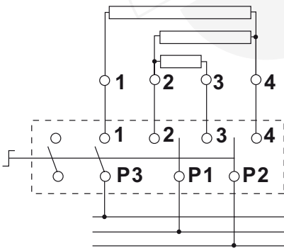
hot plate 2x3 connections 2x2-pole 4-position switch
