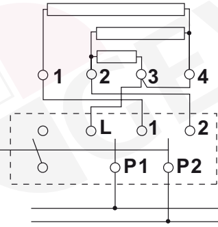
hot plate 4 connections 2-pole 4-position switch
